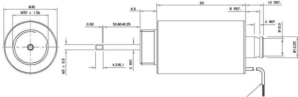
Solenoid shown in energised position
