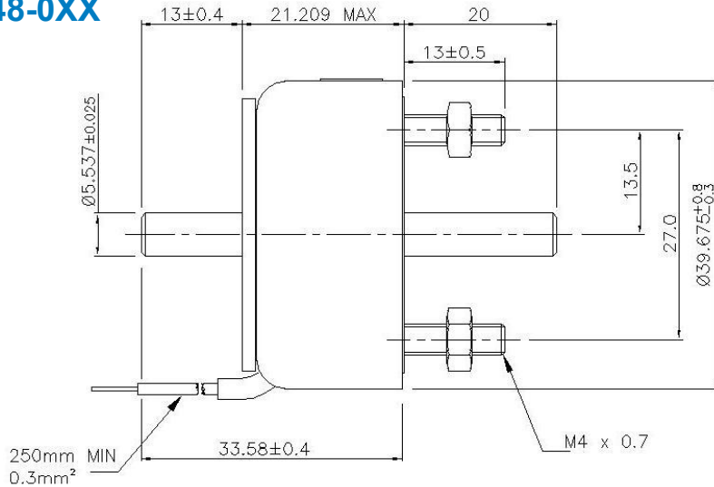
Solenoid shown in energised position
